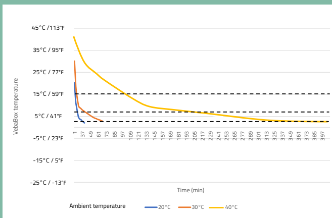
Cooling performance at different ambient temperatures >20°C / 68°F Model B Cool
