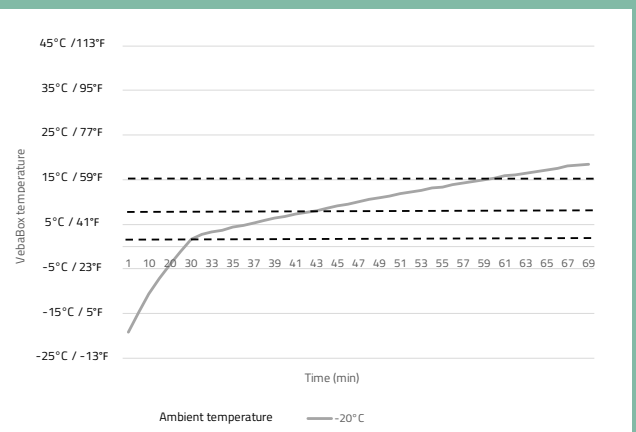
Heating performance at ambient temperature -20°C / -4°F Model B Cool
