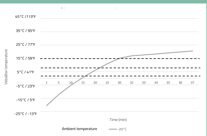
Heating performance at ambient temperature -20°C / -4°F Model C Cool
