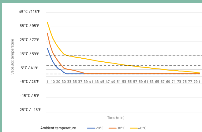
Cooling performance at different ambient temperatures >20°C / 68°F Model H Cool
