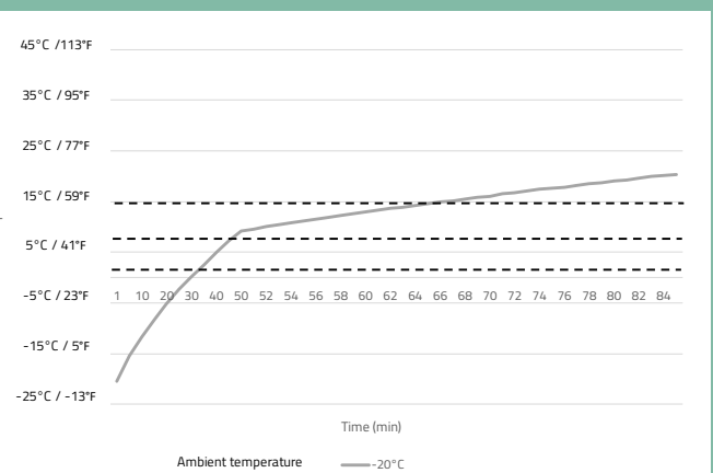
Heating performance at ambient temperature -20°C / -4°F Model H Cool
