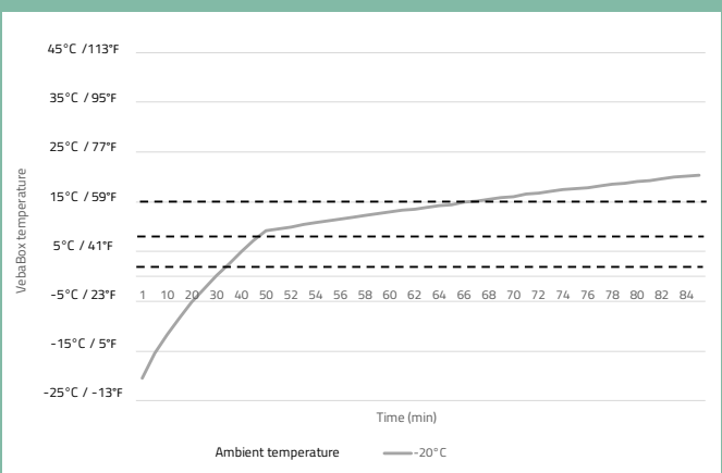
Heating performance at ambient temperature -20°C / -4°F Model O Cool
