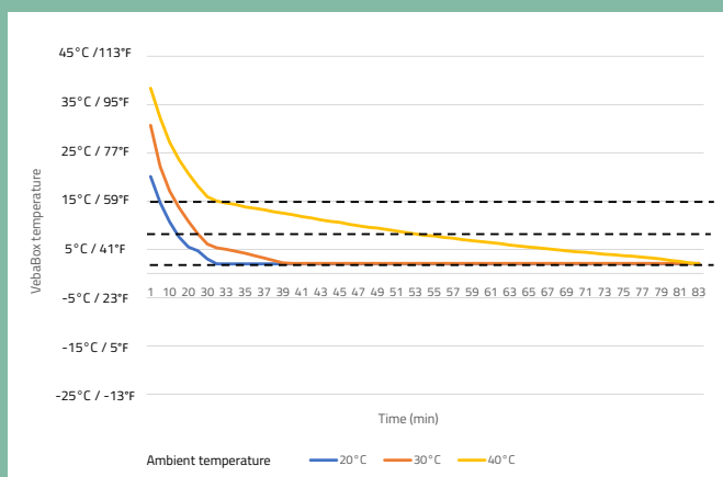
Cooling performance at different ambient temperatures >20°C / 68°F Model O Cool
