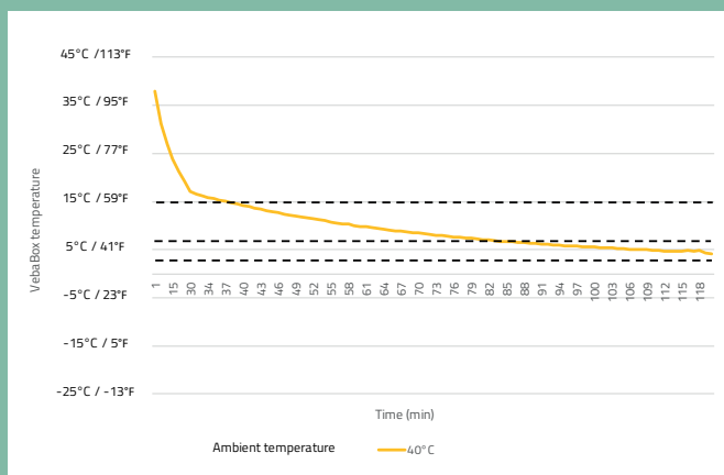
Cooling performance at ambient temperature >20°C / 68°F Model Q
