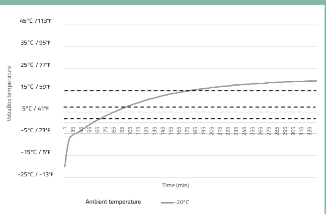
Heating performance at ambient temperature <0°C / 32°F Model Q
